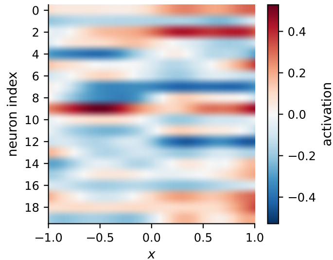
L1 (20 neurons)
