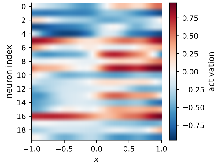
L3 (20 neurons)
