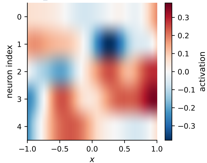
L0_quantum (5 neurons)
