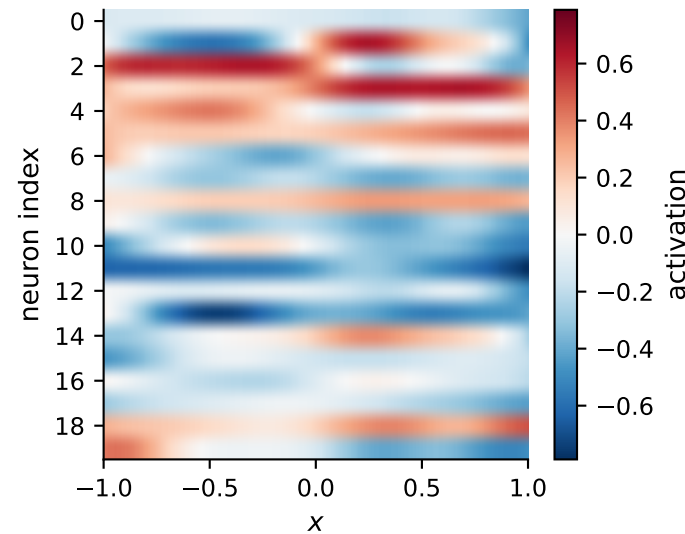
L2 (20 neurons)
